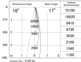
■ Direct Horizontal Illuminance DD155-2015DB9030-FX
