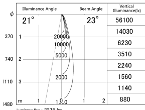
■ Direct Horizontal Illuminance DD155-2025DB9030-FX
