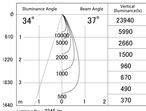
■ Direct Horizontal Illuminance DD155-2035DB9030-FX
