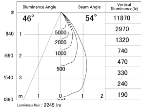
■ Direct Horizontal Illuminance DD155-2055DB9030-FX
