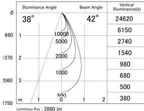
■ Direct Horizontal Illuminance DD155-2540DB9030-FX
