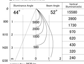
■ Direct Horizontal Illuminance DD155-2555DB9030-FX
