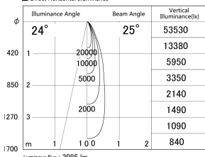
■ Direct Horizontal Illuminance DD155-3025DB9030-FX
