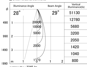
■ Direct Horizontal Illuminance DD155-3030DB9030-FX
