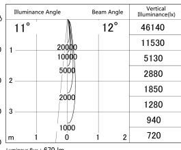
■ Direct Horizontal Illuminance DD155-0810DB9035-FX
