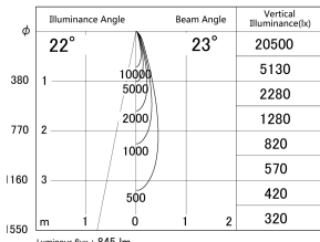
■ Direct Horizontal Illuminance DD155-0825DB9035-FX
