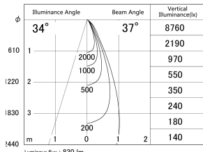
■ Direct Horizontal Illuminance DD155-0835DB9035-FX
