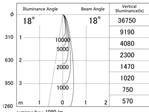
■ Direct Horizontal Illuminance DD155-1015DB9035-FX
