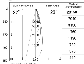
■ Direct Horizontal Illuminance DD155-1025DB9035-FX
