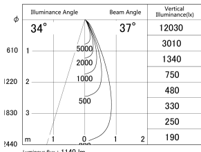
■ Direct Horizontal Illuminance DD155-1035DB9035-FX
