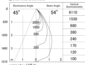
■ Direct Horizontal Illuminance DD155-1055DB9035-FX
