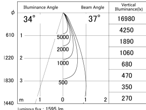
■ Direct Horizontal Illuminance DD155-1535DB9035-FX
