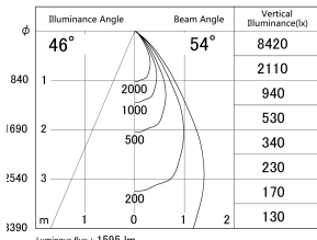
■ Direct Horizontal Illuminance DD155-1555DB9035-FX
