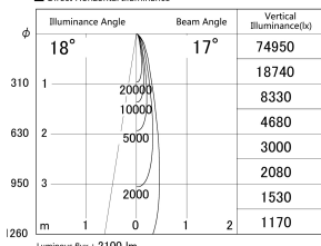
■ Direct Horizontal Illuminance DD155-2015DB9035-FX
