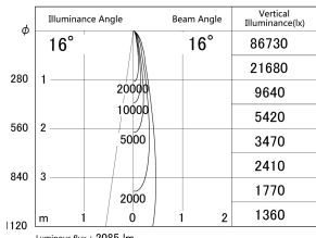
■ Direct Horizontal Illuminance DD155-2515DB9035-FX
