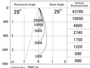
■ Direct Horizontal Illuminance DD155-2530DB9035-FX
