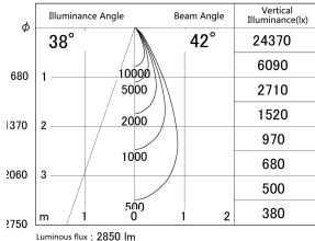
■ Direct Horizontal Illuminance DD155-2540DB9035-FX
