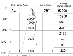
■ Direct Horizontal Illuminance DD155-3025DB9035-FX
