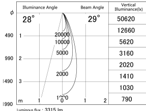
■ Direct Horizontal Illuminance DD155-3030DB9035-FX
