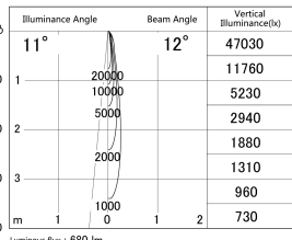
■ Direct Horizontal Illuminance DD155-0810DB9040-FX
