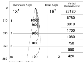
■ Direct Horizontal Illuminance DD155-0815DB9040-FX
