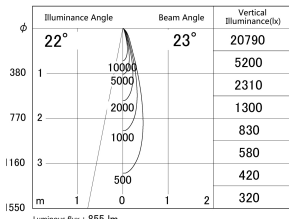
■ Direct Horizontal Illuminance DD155-0825DB9040-FX
