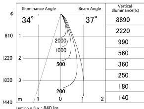
■ Direct Horizontal Illuminance DD155-0835DB9040-FX
