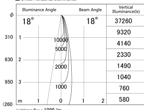
■ Direct Horizontal Illuminance DD155-1015DB9040-FX
