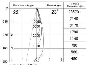
■ Direct Horizontal Illuminance DD155-1025DB9040-FX
