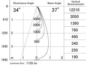
■ Direct Horizontal Illuminance DD155-1035DB9040-FX
