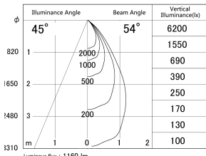
■ Direct Horizontal Illuminance DD155-1055DB9040-FX
