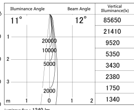
■ Direct Horizontal Illuminance DD155-1510DB9040-FX
