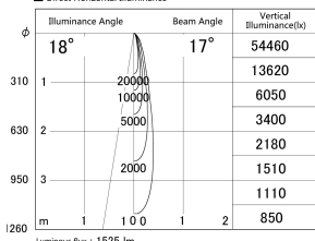
■ Direct Horizontal Illuminance DD155-1515DB9040-FX
