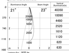
■ Direct Horizontal Illuminance DD155-1525DB9040-FX
