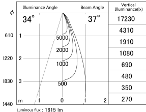
■ Direct Horizontal Illuminance DD155-1535DB9040-FX
