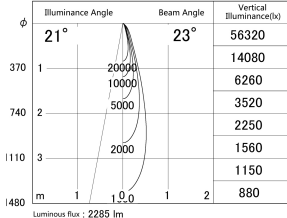
■ Direct Horizontal Illuminance DD155-2025DB9040-FX
