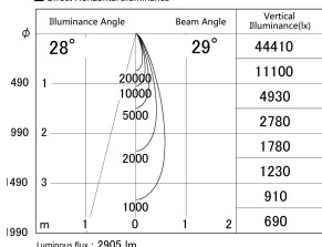
■ Direct Horizontal Illuminance DD155-2530DB9040-FX
