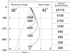
■ Direct Horizontal Illuminance DD155-2540DB9040-FX
