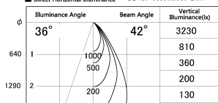
■ Direct Horizontal Illuminance DD187-0650W9030-DM1
