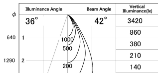
■ Direct Horizontal Illuminance DD187-0650B9040-DM1
