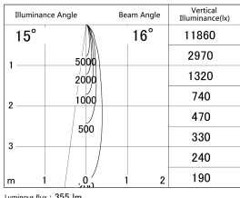
Direct Horizontal Illuminance SD278-0620W9035-DMWL
