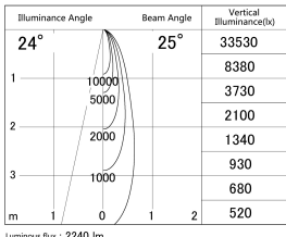
■ Direct Horizontal Illuminance SD279-2025W9030
