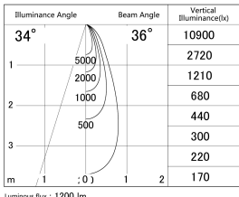
Direct Horizontal Illuminance SD279-1035B9030S
