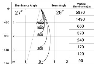
■ Direct Horizontal Illuminance SD287-0635W9027-DMWL
