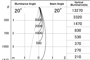
■ Direct Horizontal Illuminance SD287-0625W9030-DMWL
