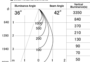
■ Direct Horizontal Illuminance SD287-0650W9035-DMWL
