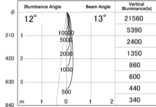
■ Direct Horizontal Illuminance SD287-0615W9040-DMWL
