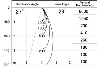
■ Direct Horizontal Illuminance SD287-0635W9040-DMWL
