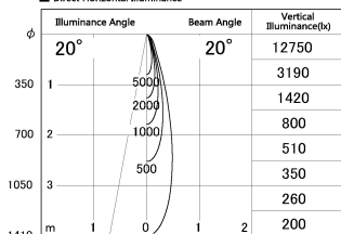
■ Direct Horizontal Illuminance SD287-0625B9027-DMWL
