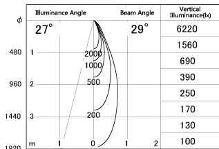
■ Direct Horizontal Illuminance SD287-0635B9030-DMWL
